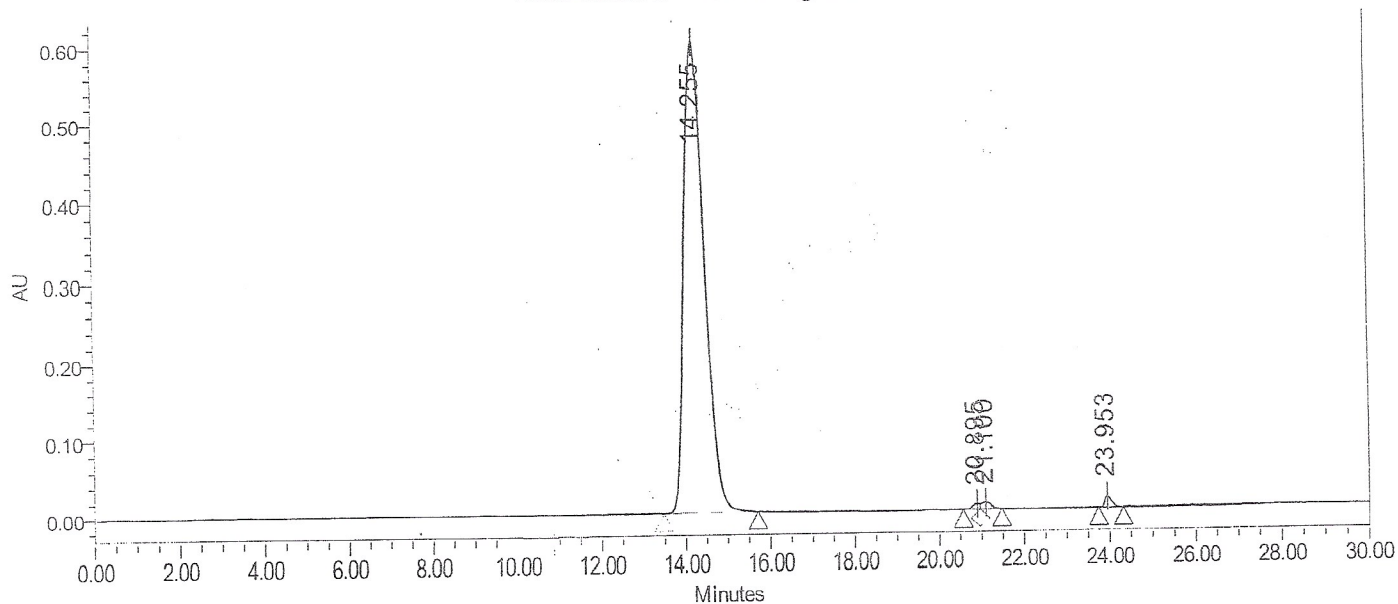
Auto-Scaled Chromatogram
